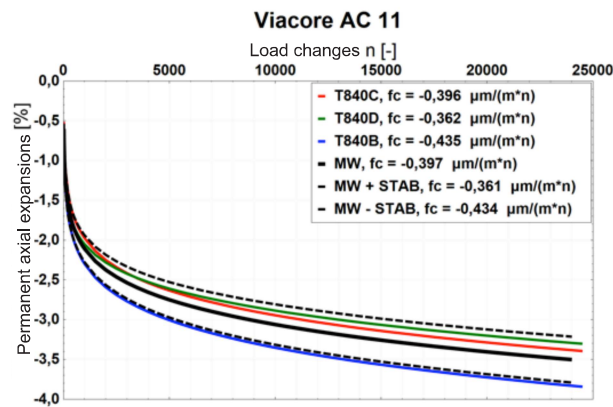
Figure 8: TCCT results for Viacore AC 11
