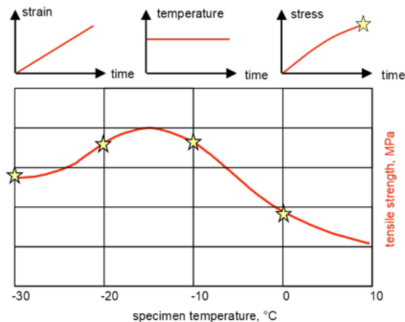
Figure 2: UTST diagram
