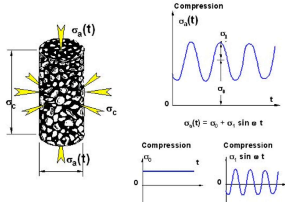
Figure 4.1: TCCT diagram
