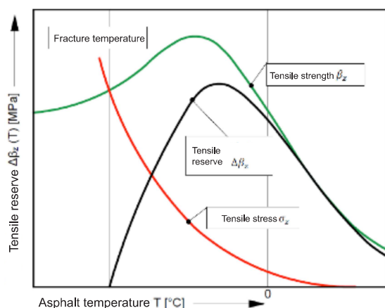
Figure 3: Tensile strength reserve
