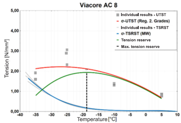
Figure 5.1: UTST and TSRST summary
